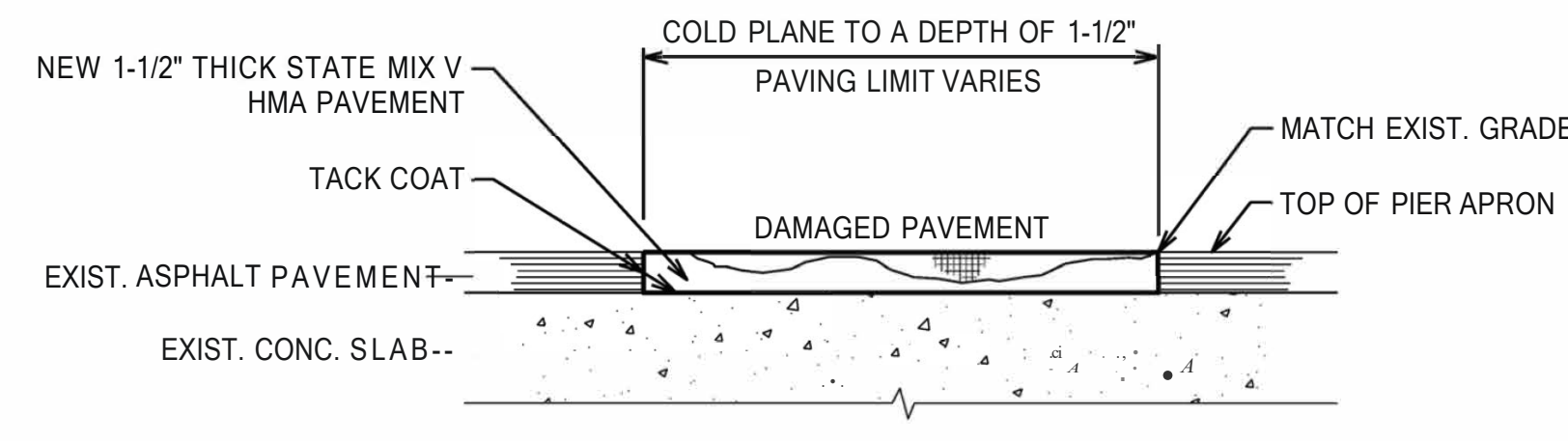
TYPE "F" REPAIR DETAIL NOTTO SCALE
