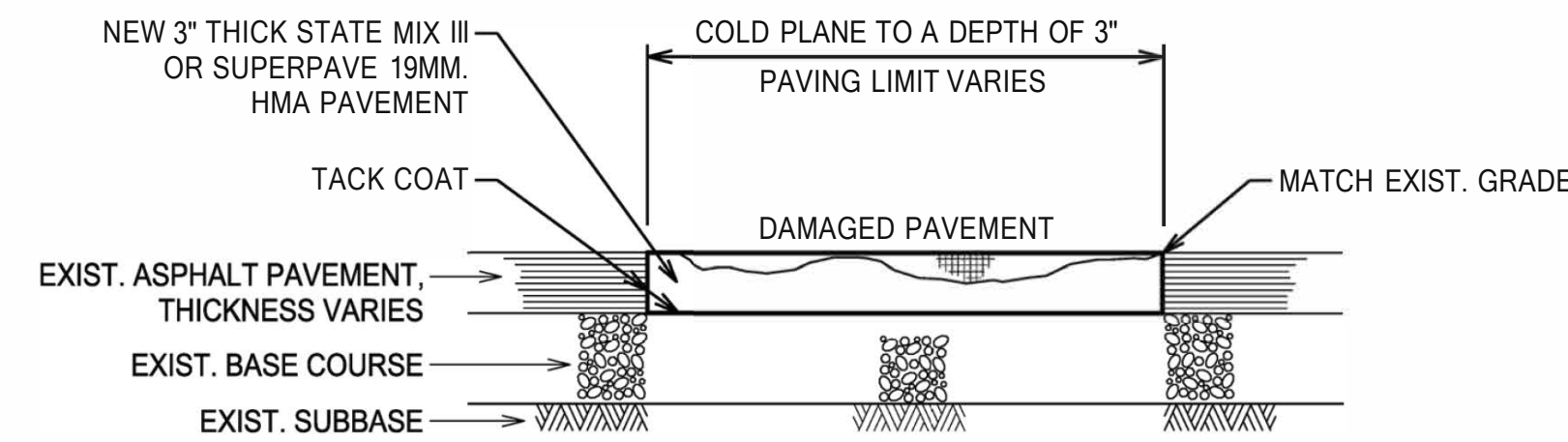
TYPE "E" REPAIR DETAIL NOTTO SCALE
