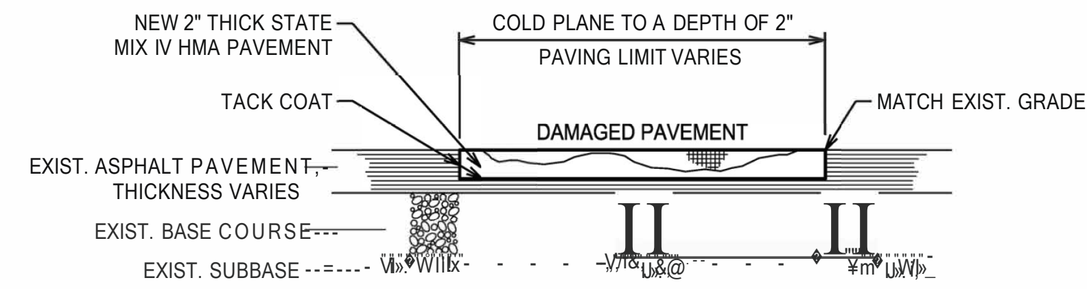
TYPE "A" REPAIR DETAIL NOTTO SCALE
