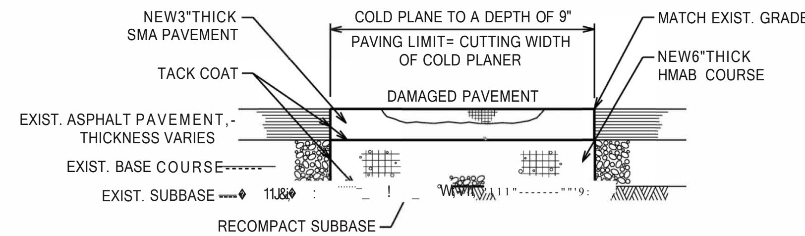
TYPE "D" REPAIR DETAIL NOTTO SCALE
