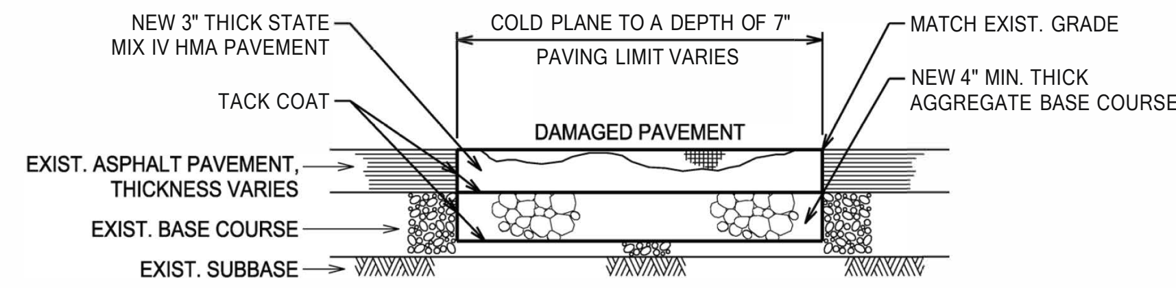
TYPE "B" REPAIR DETAIL NOTTO SCALE
