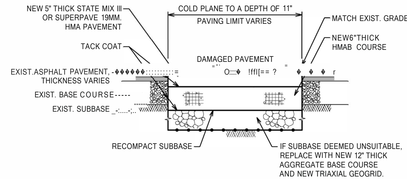
TYPE "C" REPAIR DETAIL NOTTO SCALE
